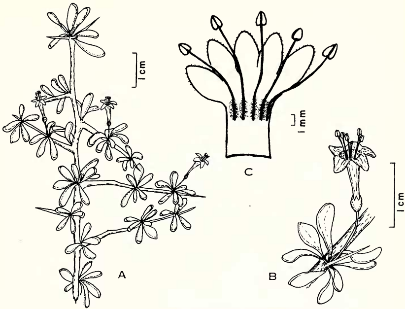
FIG. 1. Lycium arochae . A. Flowering branch. B. Enlargement of flower. C. Dissection of corolla.
